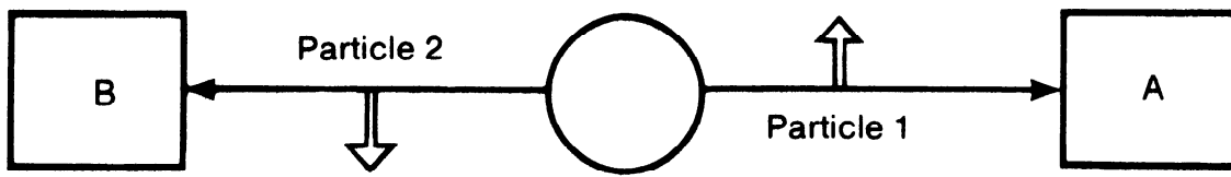
FIGURE 3.8. Spin correlation in a spin-singlet state.
