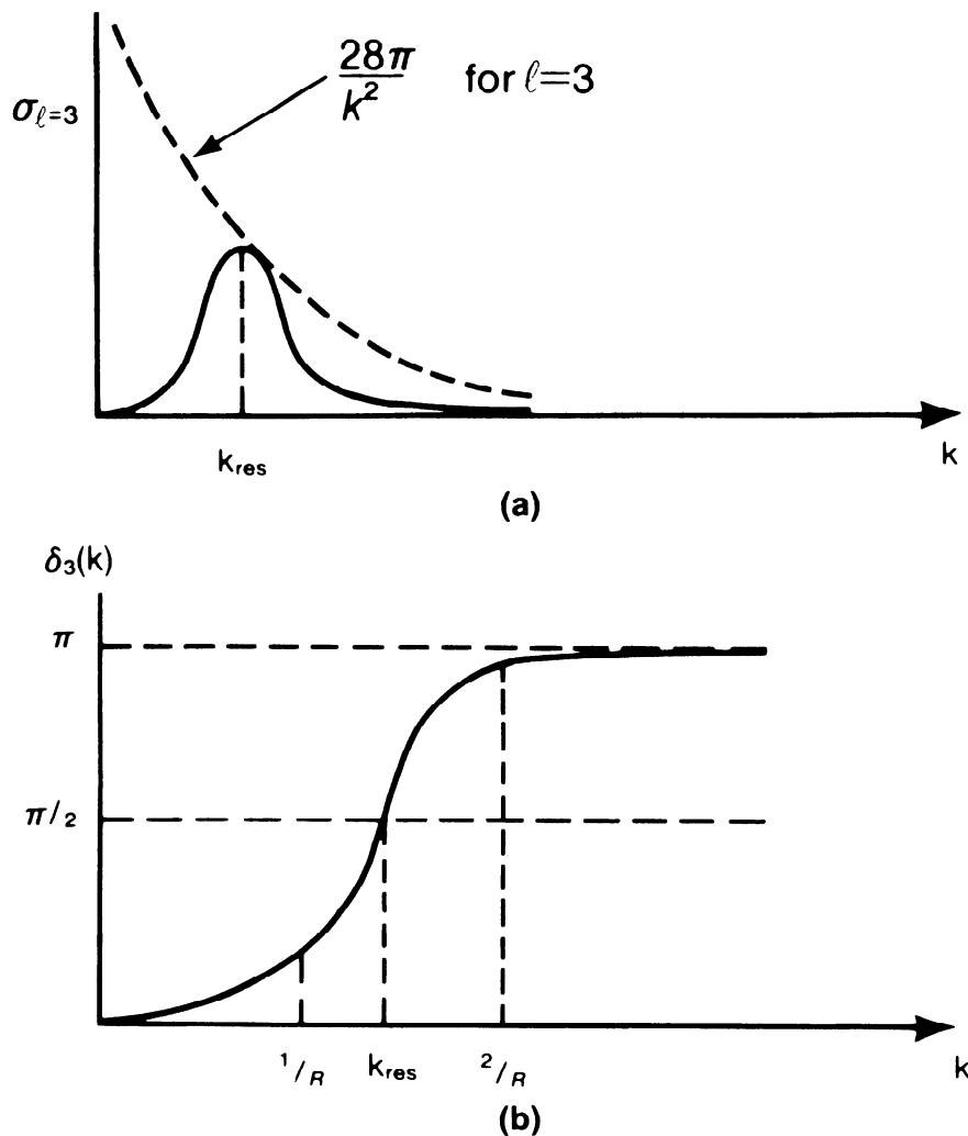
FIGURE 7.12. Plots of (a) \sigma_{l=3} versus k , where at resonance \delta_3(k_{res}) = \pi/2 and \sigma_{l=3} = (4\pi/k_{res}^2) \times 7 = 28\pi/k_{res}^2 and (b) \delta_3(k) versus k . The curves are for a spherical well with 2mV_0R^2/\hbar^2 = 5.5 .
