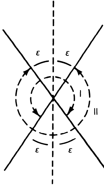
FIGURE 2.9. Regions of validity for the potentials \mathbf{A}^{(I)} and \mathbf{A}^{(II)} .
