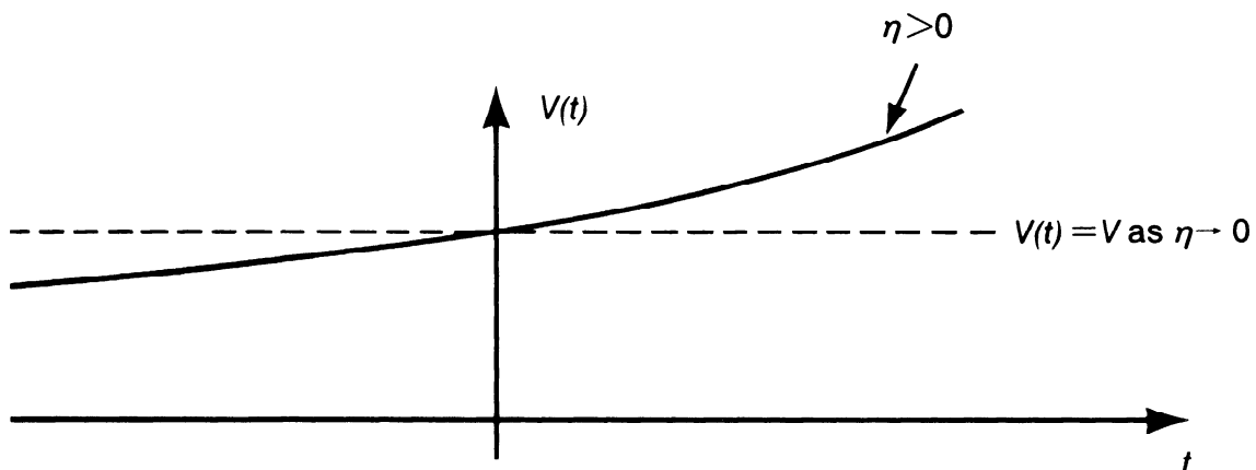
FIGURE 5.11. Plot of V(t) versus t in the adiabatic (slow-turn-on) picture.
