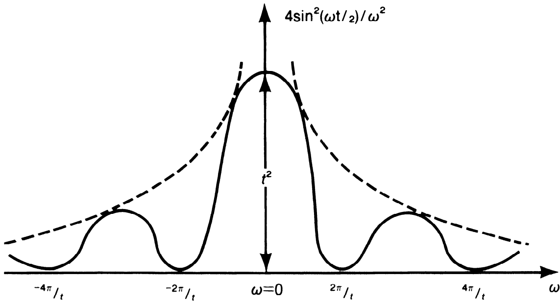
FIGURE 5.6. Plot of 4\sin^2(\omega t/2)/\omega^2 versus \omega for a fixed t , where in \omega = (E_n - E_i)/\hbar we have regarded E_n as a continuous variable.
