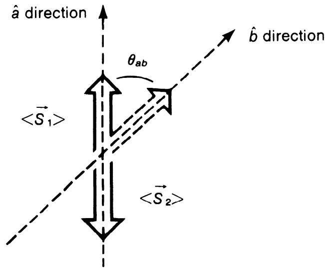
FIGURE 3.9. Evaluation of P(\hat{a}+; \hat{b}+) .
