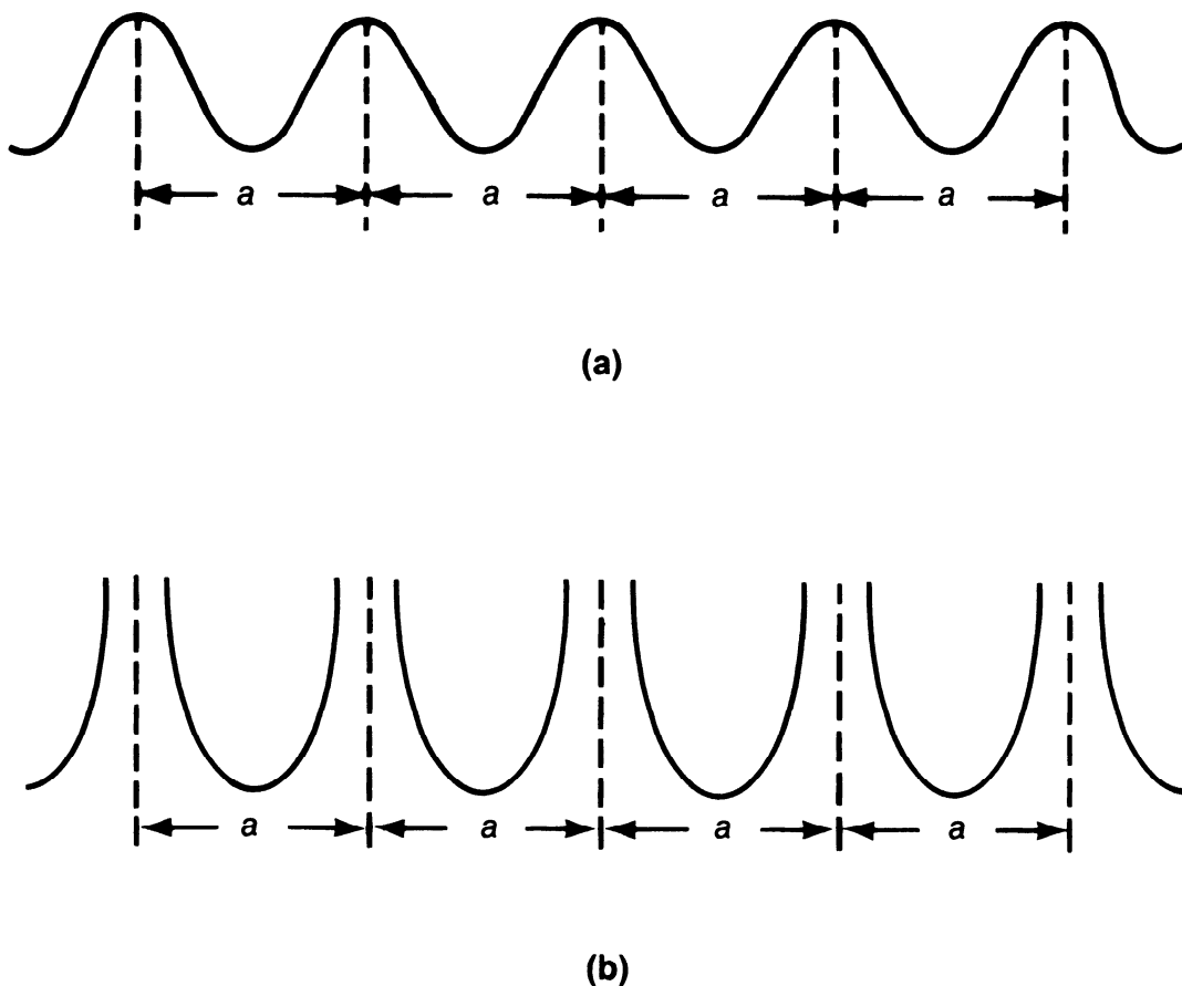
FIGURE 4.6. (a) Periodic potential in one dimension with periodicity a . (b) The periodic potential when the barrier height between two adjacent lattice sites becomes infinite.
