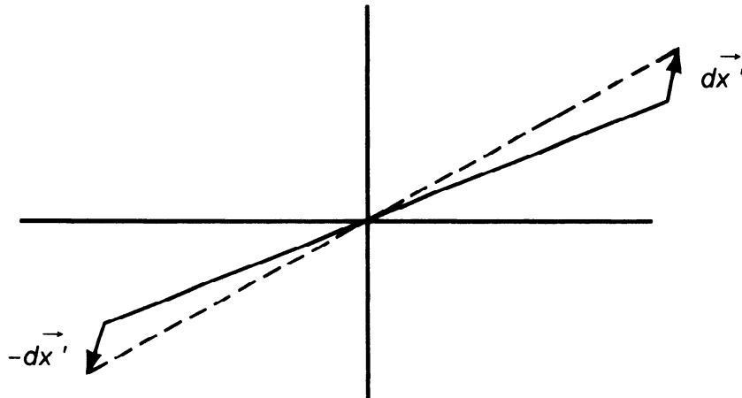
FIGURE 4.2. Translation followed by parity, and vice versa.
